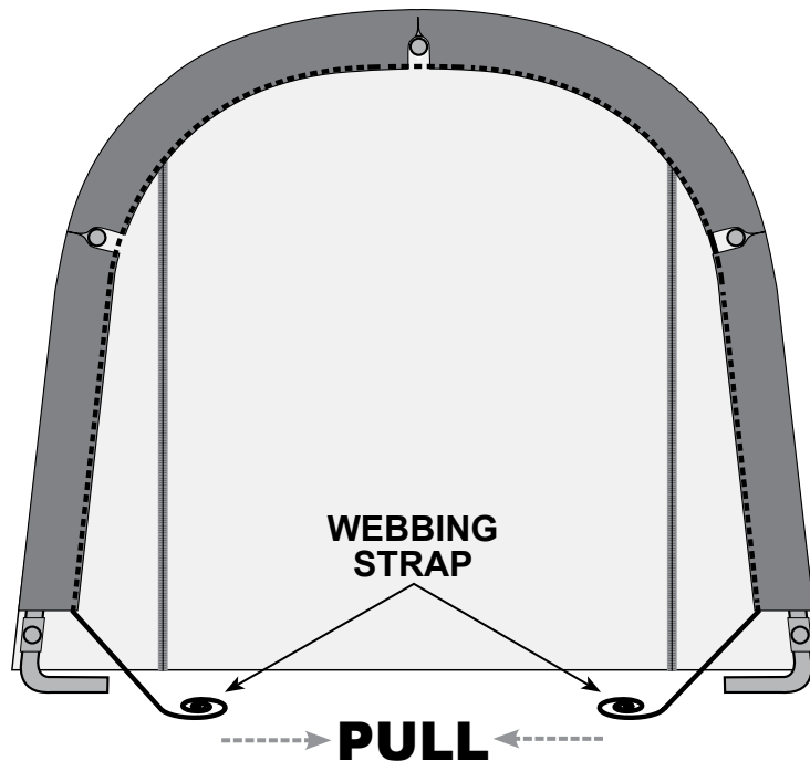
D END PANEL VIEW FROM INSIDE SHELTER
