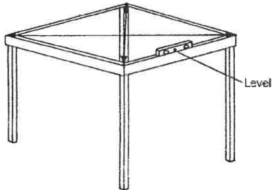
Diagonal Measurement
