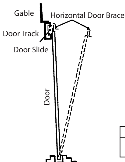
Front Frame Track
