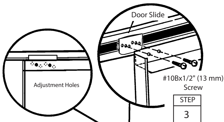
Front Frame Track
