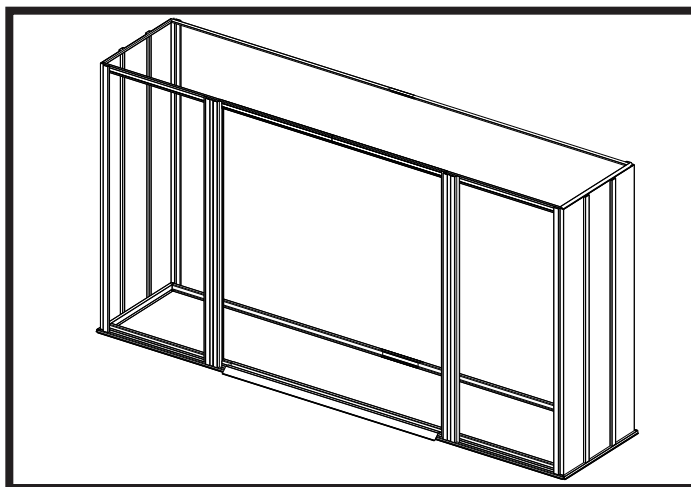
Install Corners, Wall Angles, Door Track, and Door Jamb
